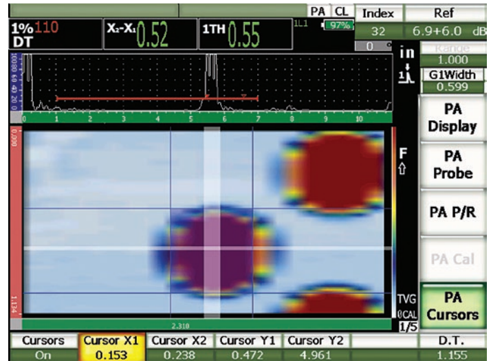
Zero-degree C-scan
