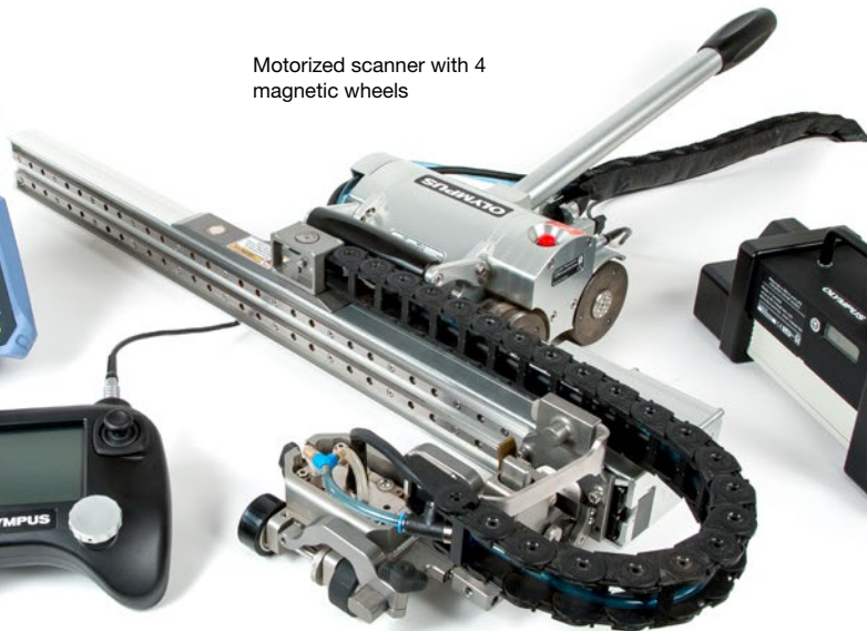
Motorized raster arm
