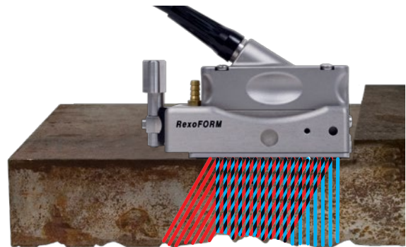
Example of beam possibilities with the RexoFORM scanner and A14 probe.
